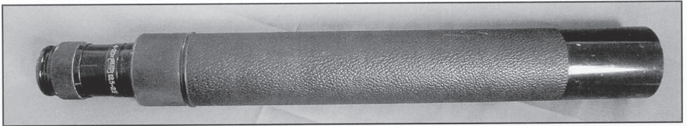
The Aseros telescope at its full length. The focusing adjustment is next to the eyepiece at left; and zooming is controlled by the ribbed ring just short of the leather-covered telescope tube. Figure 2
