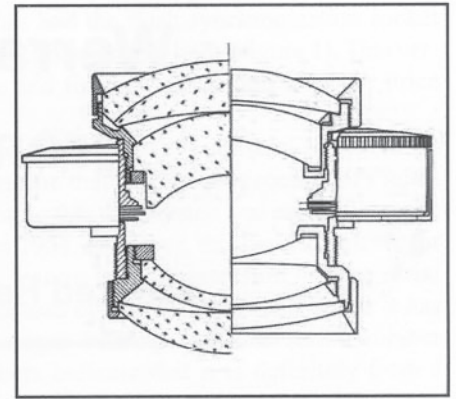
Two versions of a five-element Gaussian Planar made possible by improvements in glass technology. They are an f/2.8 80 mm lens (left) and an f/3.5 75 mm lens (right) for the 6×6 format. Figure 6
