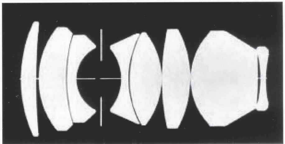
Claimed to be the world's fastest camera lens , this Planar-type f/0.7 50 mm lens was designed for NASA in the 1960s. The distance from the rear lens surface to the film plane was too small to allow space for a reflex mirror, so the lens was given a central shutter and put in a modified Hasselblad body. Figure 7
