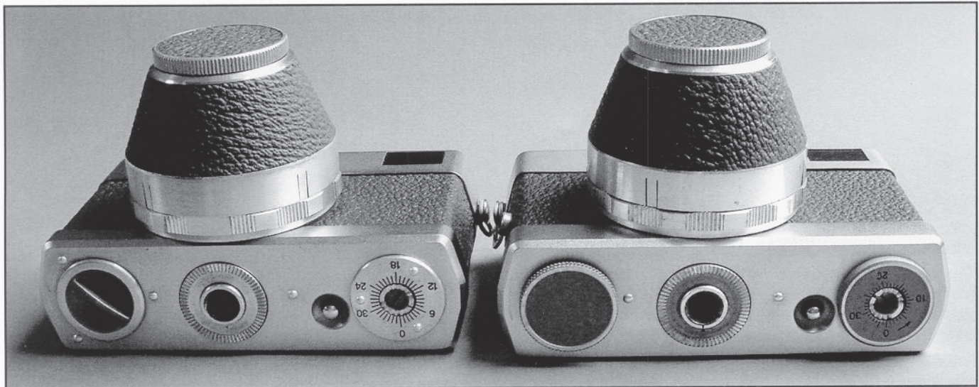
▲ Two different versions of the bottom plate for the Original Werra. Figure 10
